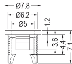
CHASSIS Ø6.4 THICKNESS 1.2
