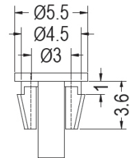
CHASSIS Ø4.5 THICKNESS 0.8
