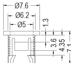
MOUNTING HOLE Ø6.4 THICKNESS 1.2
