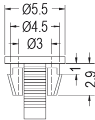
CHASSIS Ø4.5 THICKNESS 0.8
