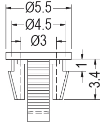
CHASSIS Ø4.5 THICKNESS 1.0
